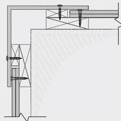
Exterior corner with corner element
