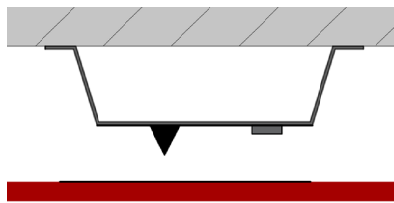
At the centre Min. width of batten is 70 mm
