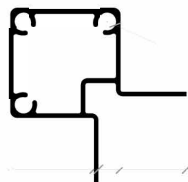
Corner profile CP 15-25-40
