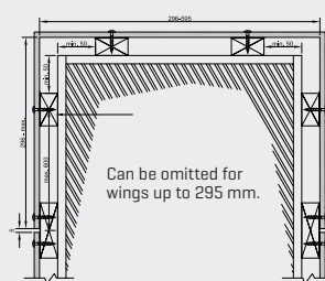
Bottom from 296 to 595 mm.
