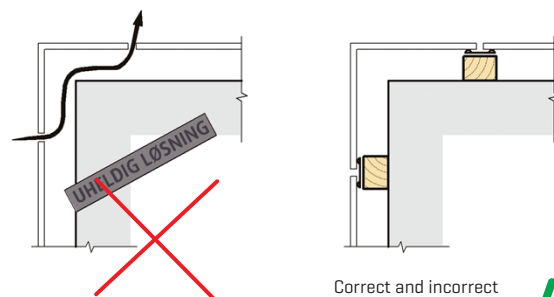
Two-stage sealing principle
