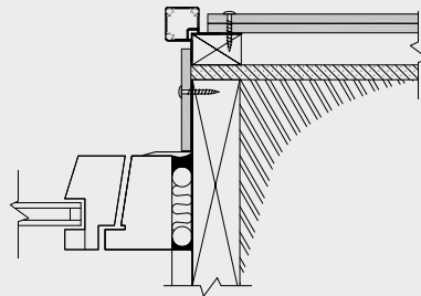
Edge along windows with corner profile CP-15-25-40
